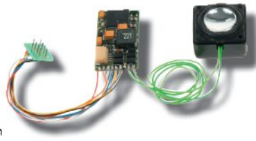
36 020/36 420 Sound decoder with 8-way NEM 652 plug
